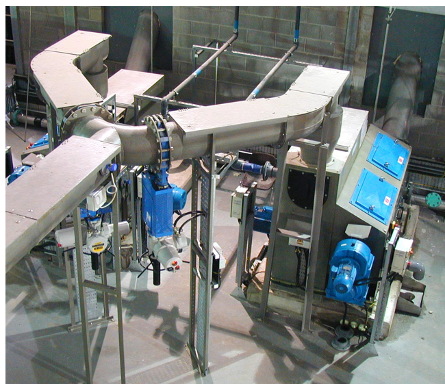
Laundry with Bifurcated y Branch and Actuated Knife Gate Valves
